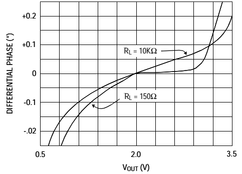
Differential Phase for R_L Tied to 0V R_F = 1KΩ, A_V = +2
