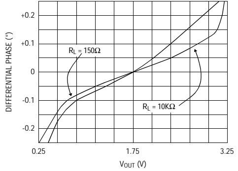
Differential Phase for R_L Tied to 2.5V R_F = 0, A_V = +1
