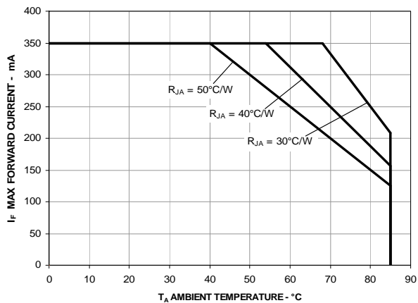
Figure 5. Maximum forward current vs. ambient temperature Derated based on T_{JMAX} = 110^{\circ}\text{C} , R_{\theta JA} = 30^{\circ}\text{C/W} / 40^{\circ}\text{C/W} and 50^{\circ}\text{C/W}
