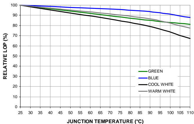
Figure 9: Relative LOP vs. junction temperature
