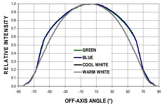
Figure 4: Radiation Pattern
