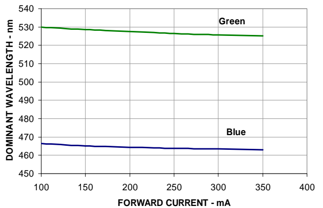
Figure 6: Dominant wavelength vs. forward current – InGaN devices
