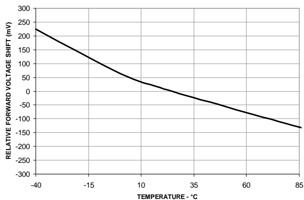
Figure 8: Temperature vs. relative forward voltage shift
