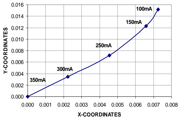
Figure 7: Chromaticity Shift vs. Current *Note: (x,y) values @ 350mA reference to (0.0)
