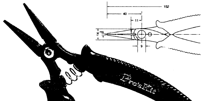
1PK-5102-E With Conductive Handle
