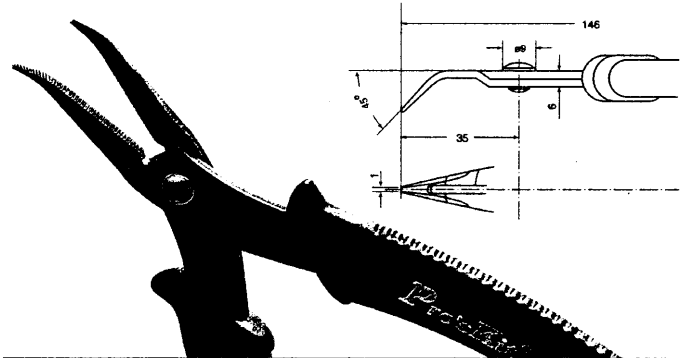
1PK-105-E With Conductive Handle
