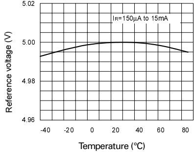
Temperature Drift
