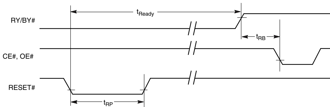
Figure 16. Reset Timings
