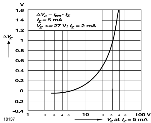
Figure 14. Change of Zener voltage from turn-on to the point of thermal equilibrium vs. Zener voltage
