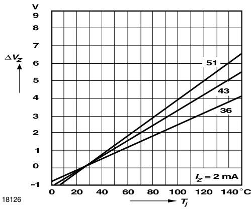
Figure 13. Change of Zener Voltage vs. Junction Temperature
