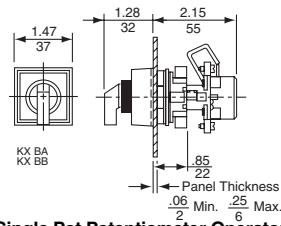
Single Pot Potentiometer Operator
