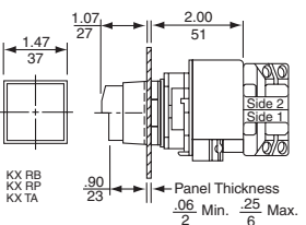
Single Push Button Operator Illuminated
