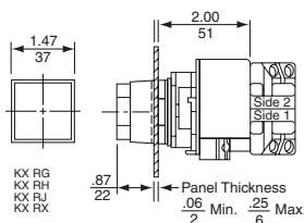
Dual Push Button Operator Illuminated
