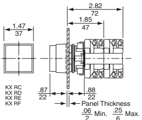
Dual Push Button Operator Non-Illuminated
