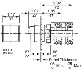
Single Push Button Operator Non-Illuminated
