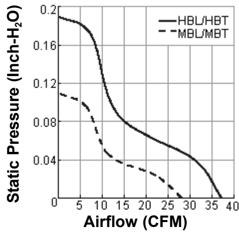
Ball (60Hz)
