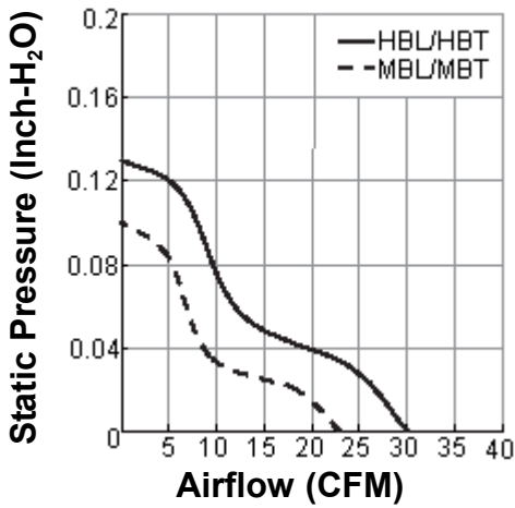
Ball (50Hz)
