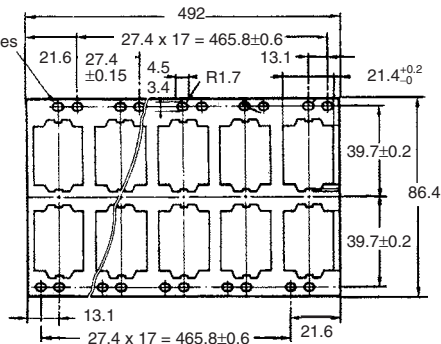
PYP-36 (for Mounting 36 Sockets)
