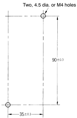
Mounting Holes
