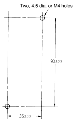
Mounting Holes
