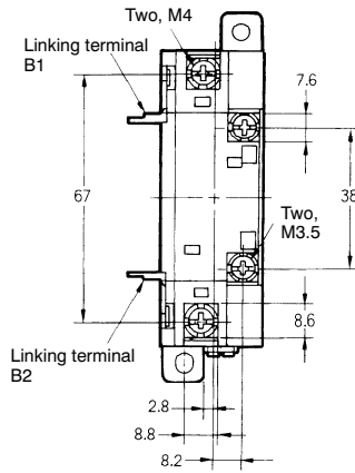
Terminal Arrangement/ Internal Connections
