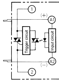
Terminal Arrangement/ Internal Connections
