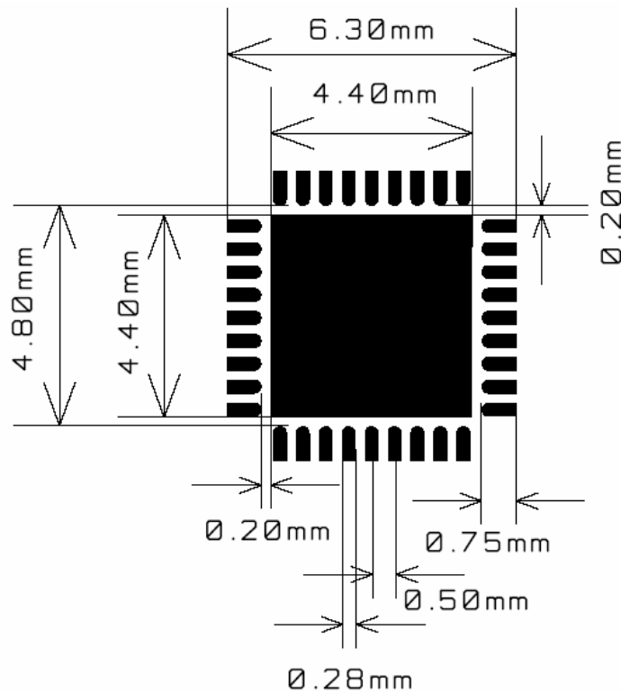
Figure 62: Recommended PCB Layout for QLP 36 Package
