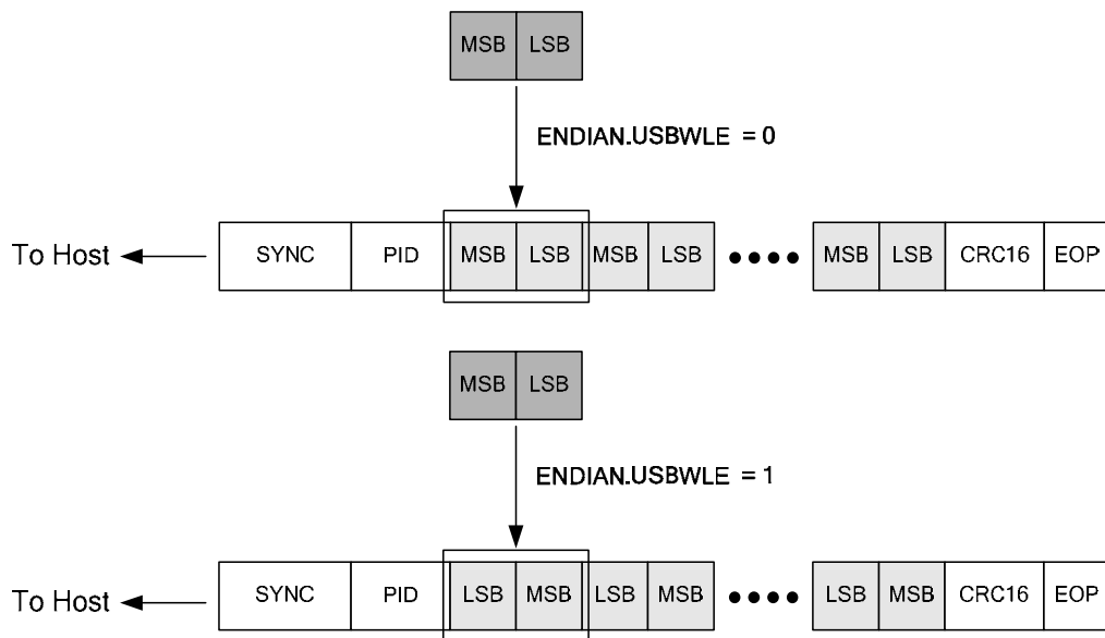
Figure 45: Writing Big/Little Endian
