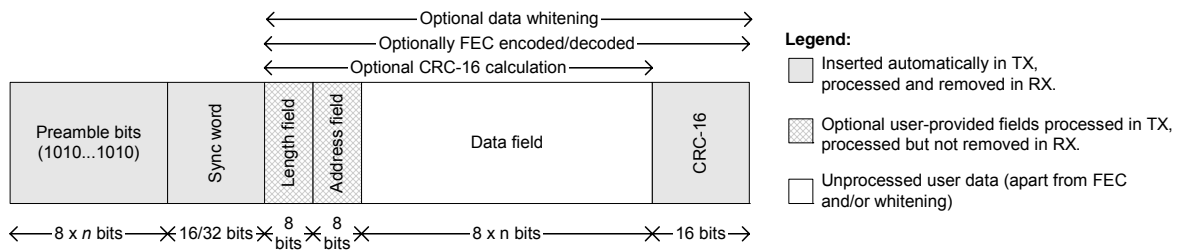
Figure 51: Packet Format
