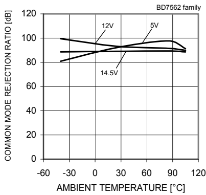
Fig.19 Common Mode Rejection Ratio – Ambient Temperature ( V_{DD}=12[V] )
