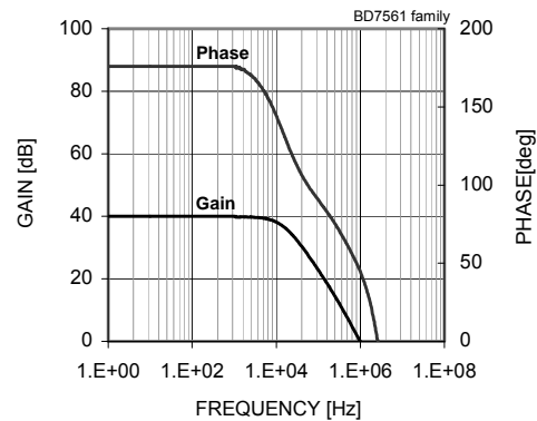
Fig.23 Gain - Frequency
