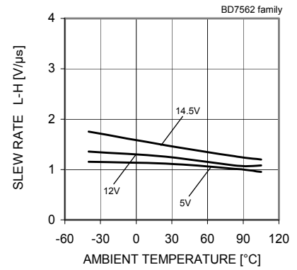
Fig.21 Slew Rate L-H – Ambient Temperature
