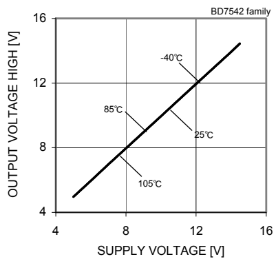
Fig.5 Output Voltage High - Supply Voltage ( R_L=10[k\Omega] )
