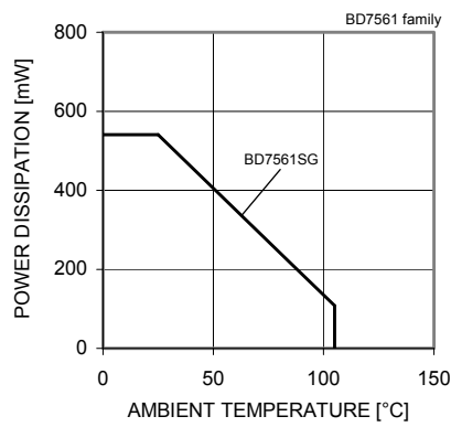
Fig.2 Derating Curve
