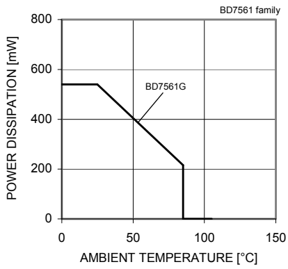
Fig.1 Derating Curve
