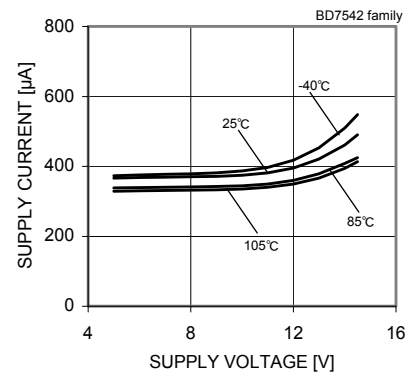
Fig.3 Supply Current - Supply Voltage
