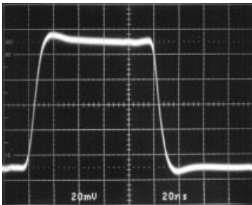
R_F = R_G = 1\text{k} V_{IN} = 100\text{mV} LT1220 • TPC22 V_S = \pm 15\text{V} f = 5\text{MHz}
