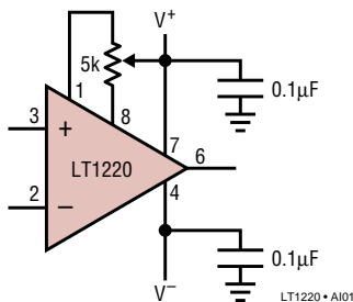
LT1220 • A101
