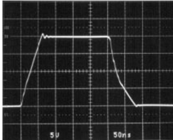
R_G = 0 V_{IN} = 20\text{V} LT1220 • TPC20 V_S = \pm 15\text{V} f = 2\text{MHz}
