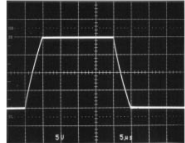
R_G = 0 V_{IN} = 10\text{V} LT1220 • TPC21 V_S = \pm 15\text{V} f = 20\text{kHz}
