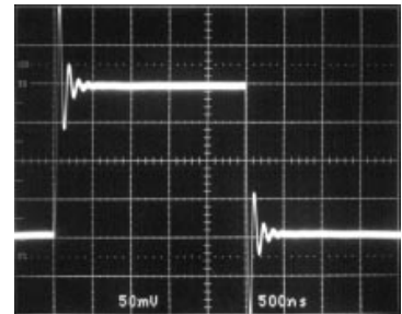
R_F = R_G = 1\text{k} V_{IN} = 200\text{mV} LT1220 • TPC24 V_S = \pm 15\text{V} f = 200\text{kHz}
