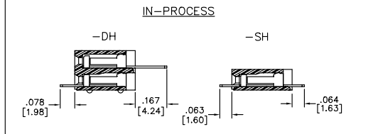
FIGURE 2 HORIZONTAL MOUNT
