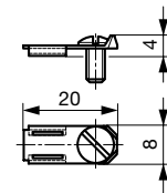
Screw-Adapter for Quick Connect-Terminals 6.3 x 0.8 mm
