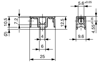
Reflow-Cover with Clamp 0853.0576
