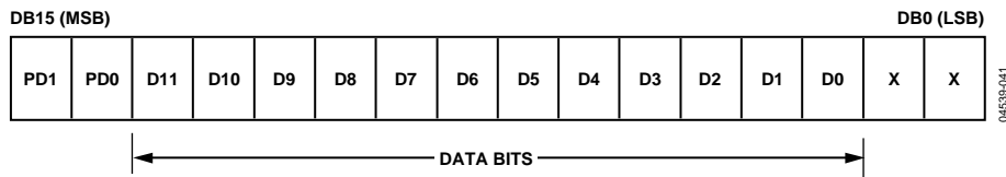
Figure 40. AD5620 Input Register Contents
