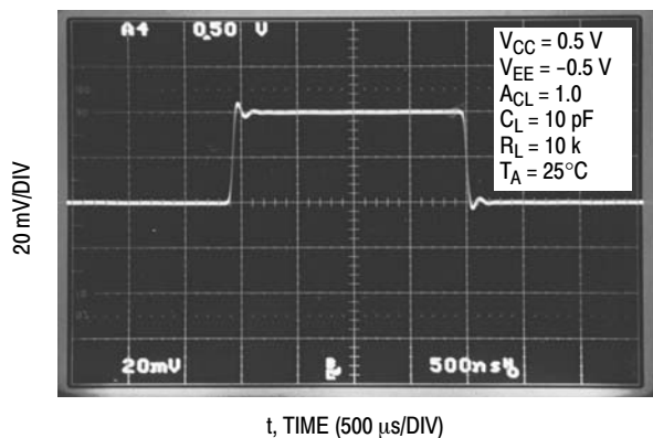
Figure 7. Transient Response
