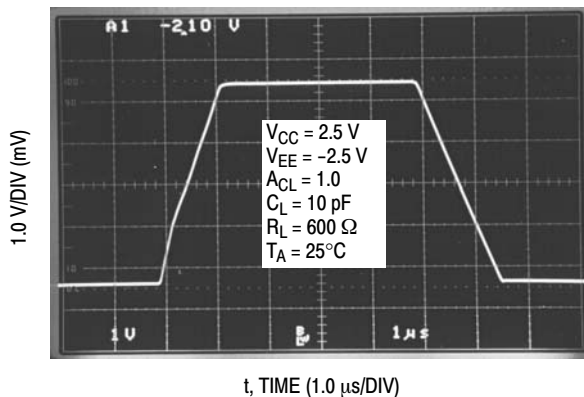
Figure 8. Slew Rate
