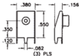
Mounting Detail
