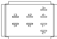
18 switching element for emergency stop switch page 447
