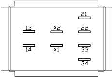
16 switching element for illuminated-/pushbutton, keylock-/selector switch 2 positions page 446
