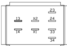
7 switching element for illuminated-/pushbutton, keylock-/selector switch 2 positions page 446
