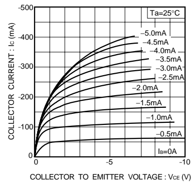
Fig.10 Grounded emitter output characteristics (II)
