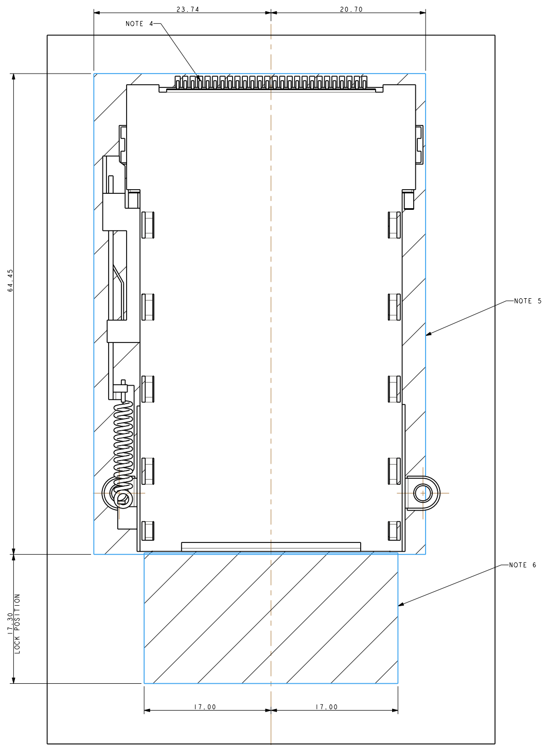
GUIDERAIL AND CONNECTOR MOUNTED ON A PCB
