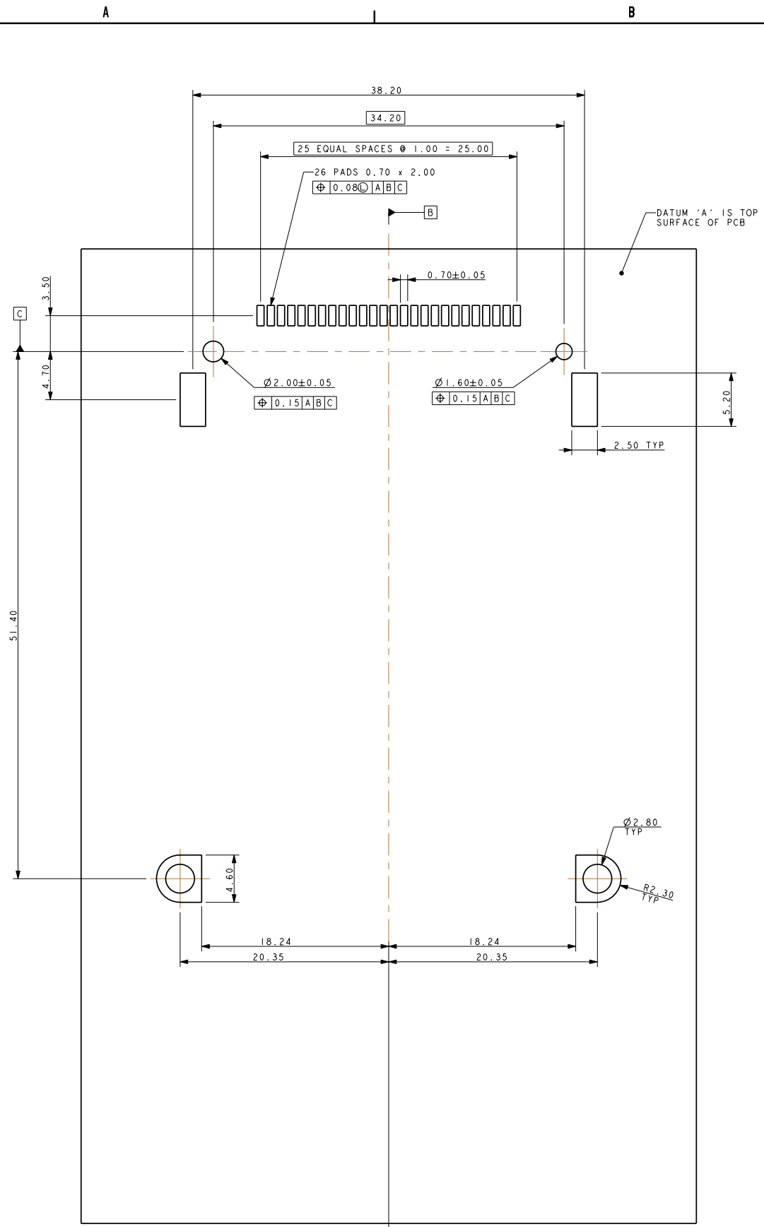
SUGGESTED PCB LAYOUT
