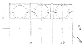
panel cutout
