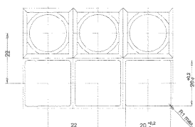
panel cutout
