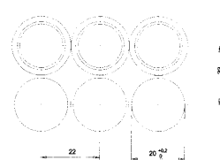
panel cutout
