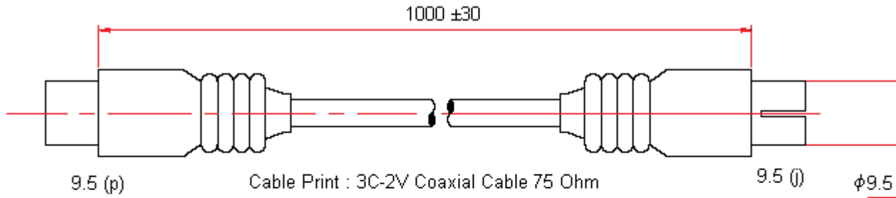
Wiring Diagram
