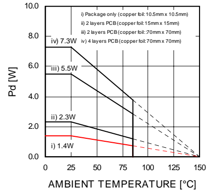
Fig.45 Thermal derating curve (HRP7)
