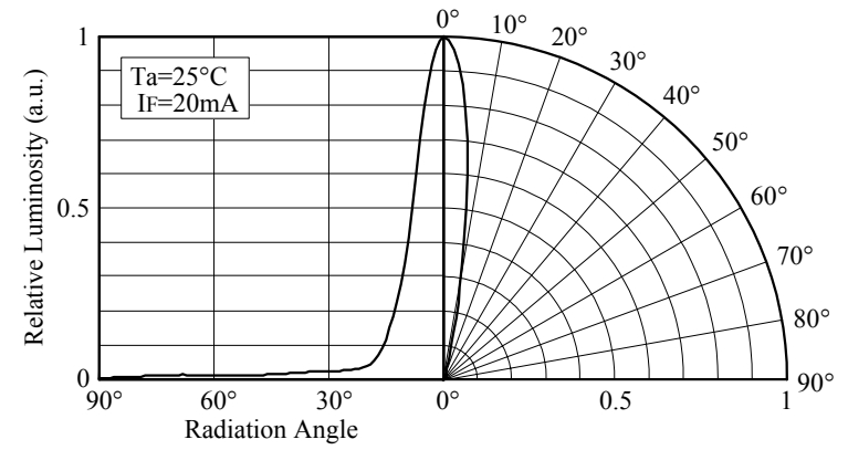
■ Directivity (NSPB500(S))
