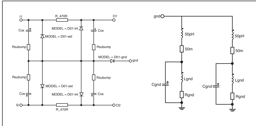
Figure 9. Aplac model
