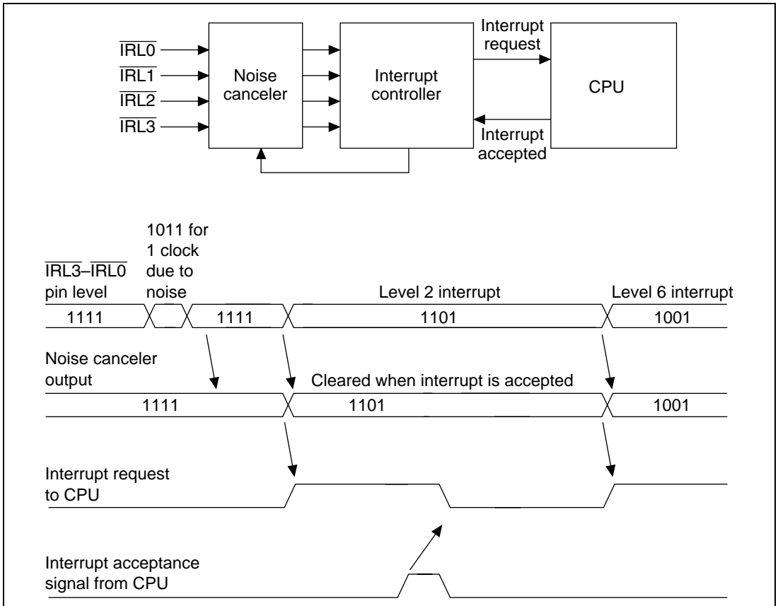
Figure 5.10 \overline{\text{IRL3}} to \overline{\text{IRL0}} Pin Sampling
