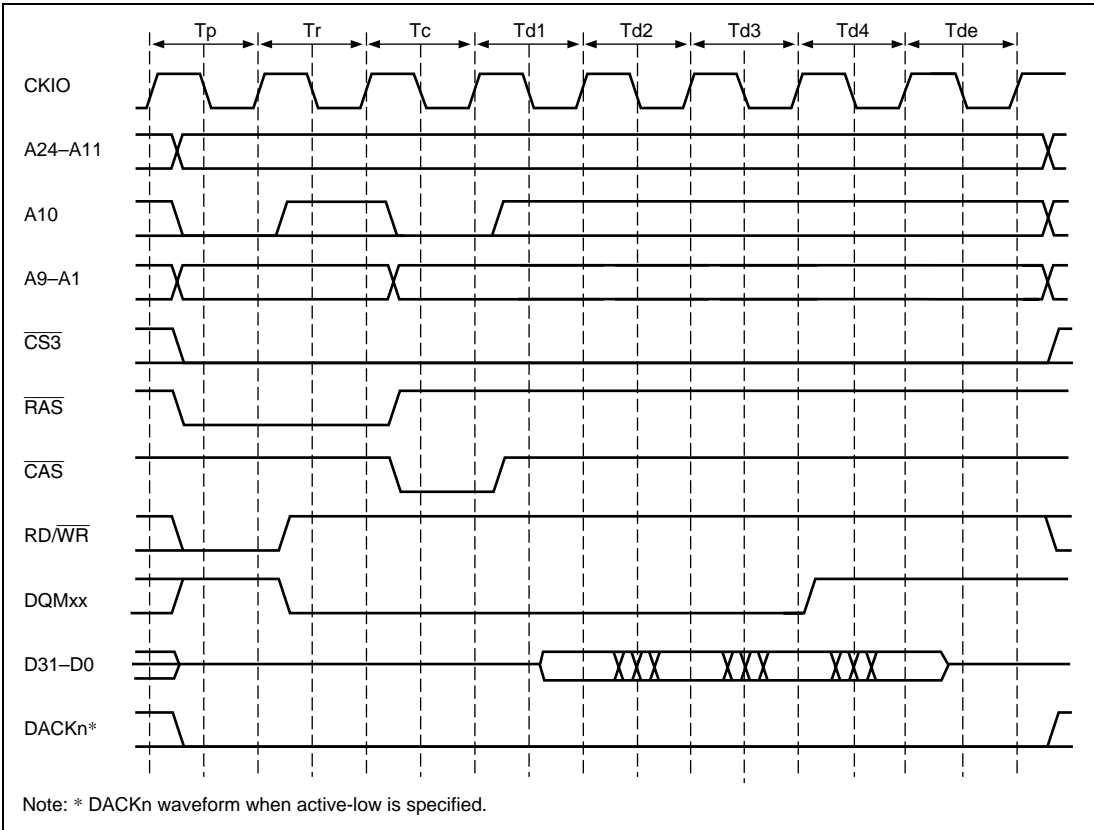
Figure 7.26 (a) Burst Read Timing (Bank Active, Different Row Addresses) Except t_{E_{eye}}:t_{P_{eye}} 1:1
