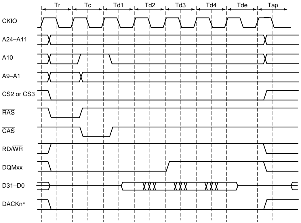
Figure 7.21 (a) Single Read Timing (Auto-Precharge) Except t_{Eyc} : t_{Pec} 1:1
