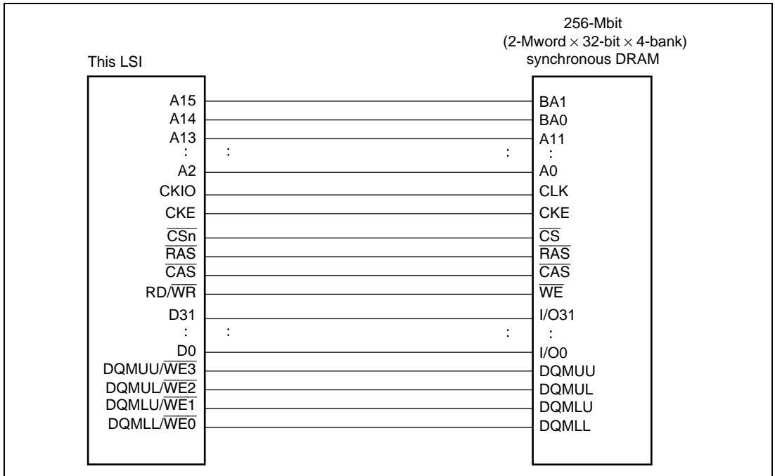
Figure 7.37 256-Mbit Synchronous DRAM (8 Mwords \times 32 Bits) Connection Example
