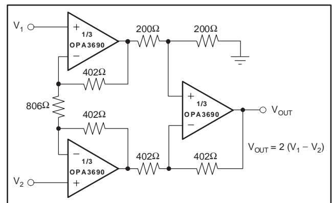
Figure 6. Instrumentation Amplifier
