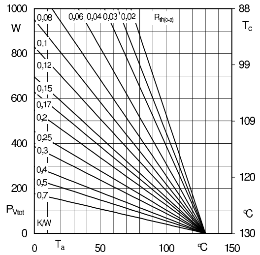
Fig. 4R: Max. power dissipation of three modules vs. case temperature
