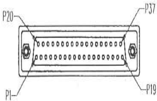
J2-DB37P FEMALE
