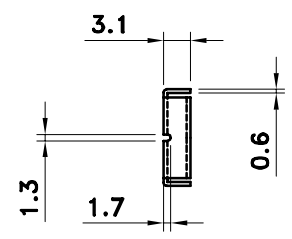
FLAT WASHER
