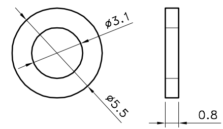
FLAT WASHER
