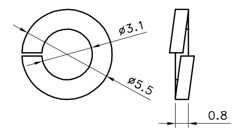
SPLIT WASHER
