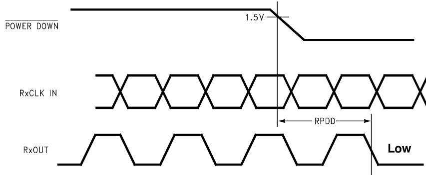
FIGURE 14. Receiver Powerdown Delay
