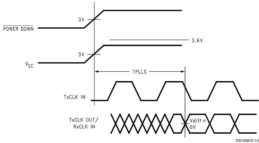
FIGURE 10. DS90CR287 (Transmitter) Phase Lock Loop Set Time
