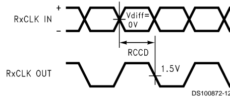
FIGURE 9. DS90CR288 (Receiver) Clock In to Clock Out Delay
