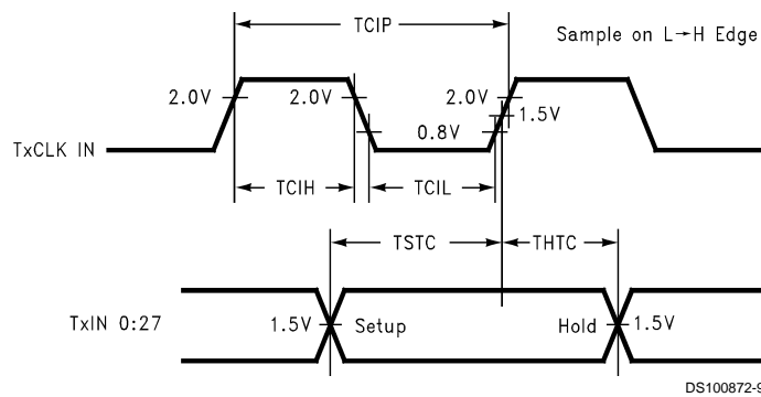
FIGURE 6. DS90CR287 (Transmitter) Setup/Hold and High/Low Times
