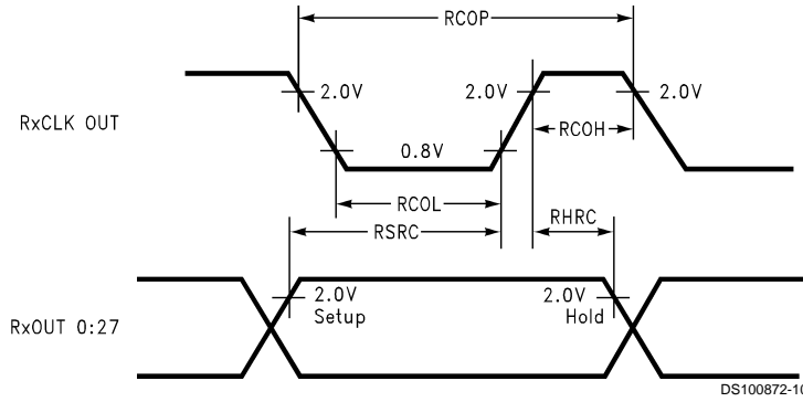
FIGURE 7. DS90CR288 (Receiver) Setup/Hold and High/Low Times
