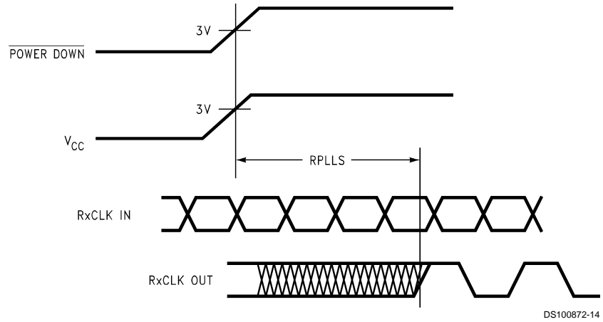
FIGURE 11. DS90CR288 (Receiver) Phase Lock Loop Set Time
