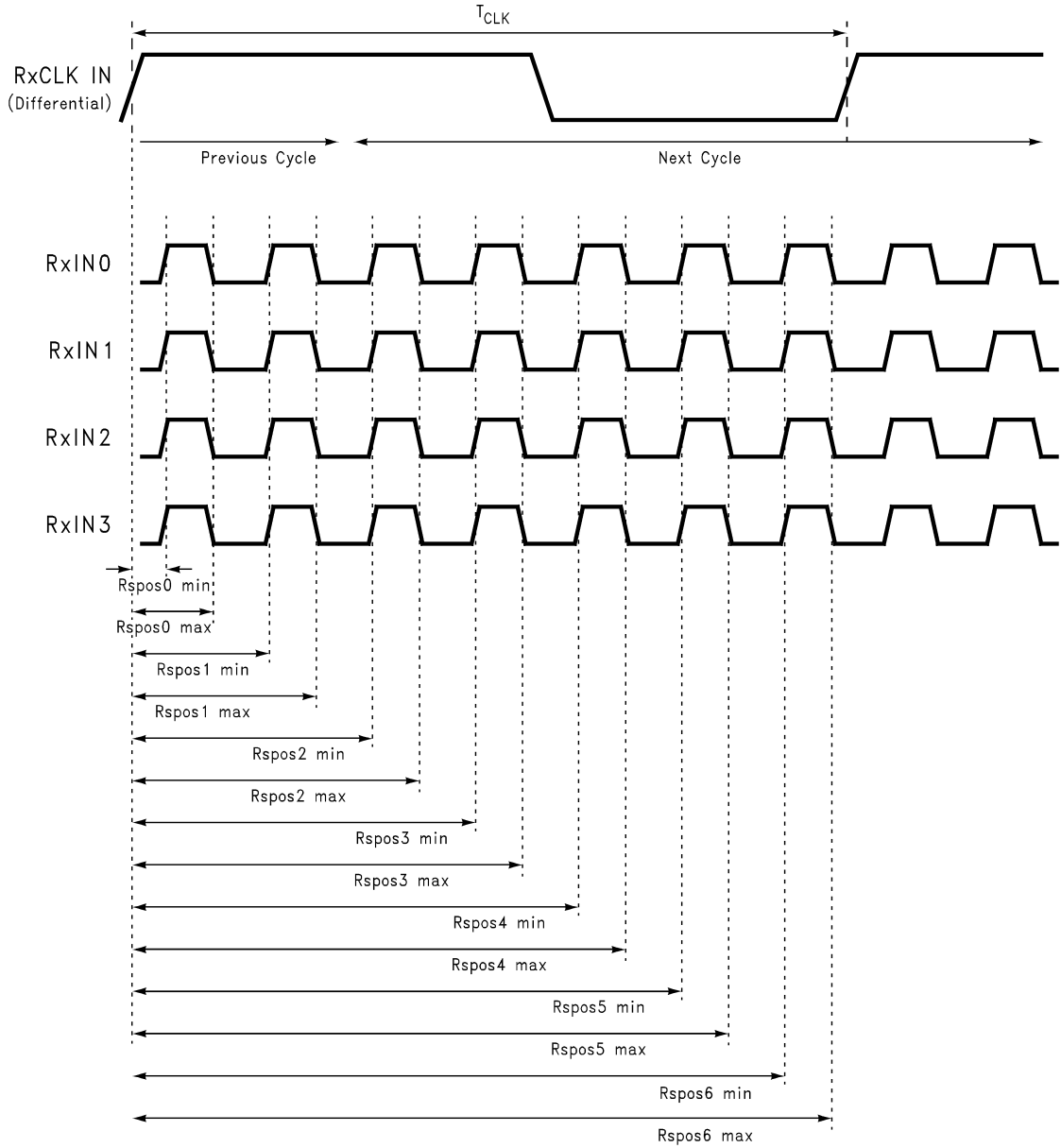
FIGURE 16. Receiver LVDS Input Strobe Position
