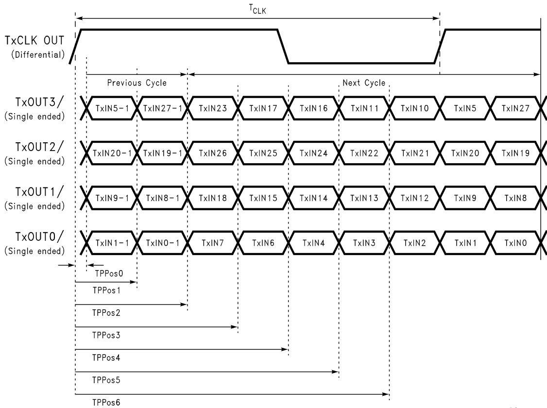
FIGURE 15. Transmitter LVDS Output Pulse Position Measurement
