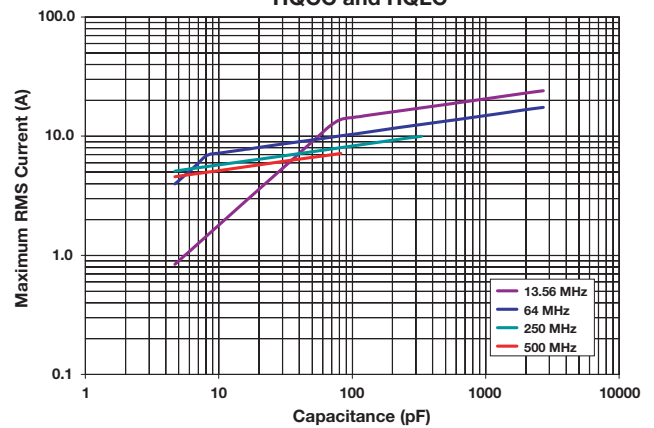
Maximum RMS Current vs. Capacitance HQCC and HQLC
