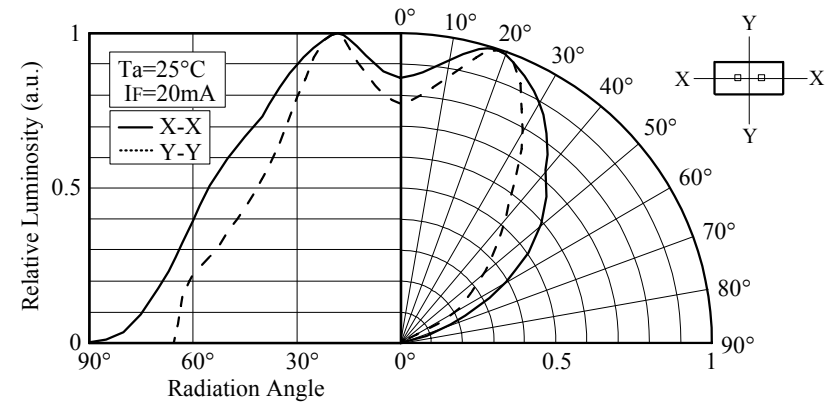
■ Directivity (NSPGF50S)
