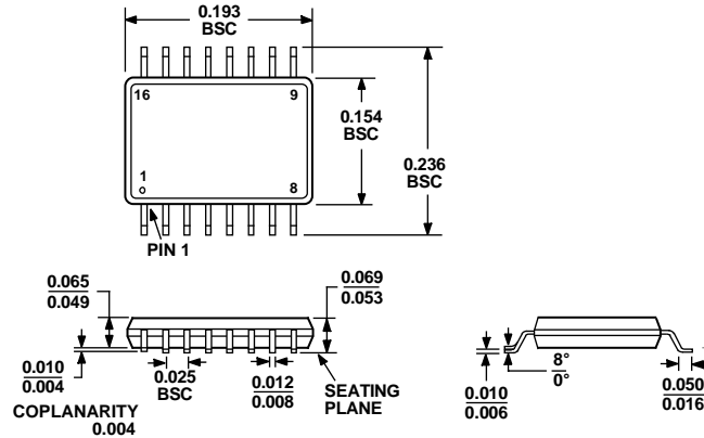
Figure 45. 16-Lead Shrink Small Outline Package [QSOP] (RQ-16) Dimensions shown in inches
