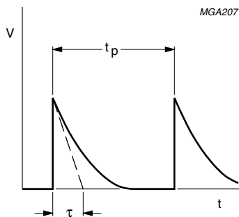
Fig. 15 Exponential pulses
