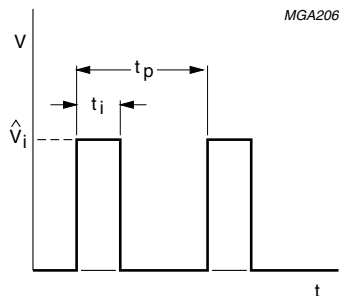
Fig. 14 Rectangular pulses
