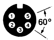
5A pole 60° contact spacing
