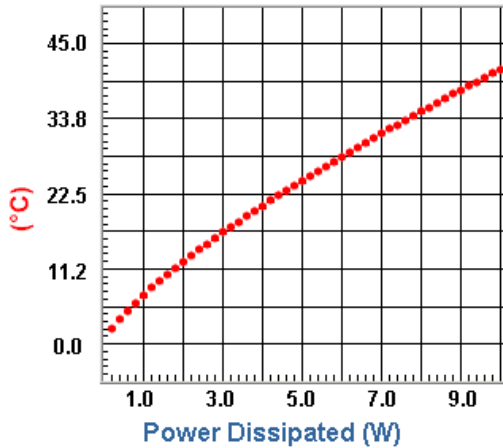
Heat Sink Temperature Rise Above Ambient
