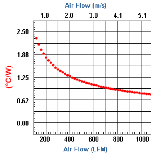
Heat Sink Thermal Resistance
