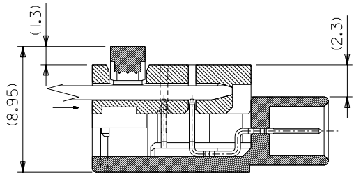
SECT B-B (SCALE:4-1)
