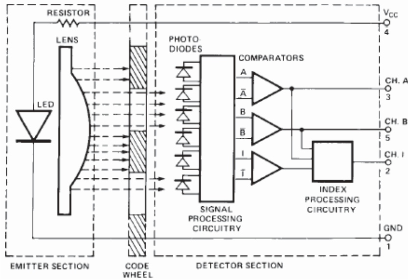
Figure 1. Block Diagram
