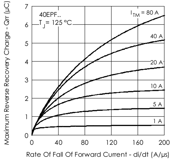
Fig. 11 - Recovery Charge Characteristics, T_J = 125^\circ\text{C}
