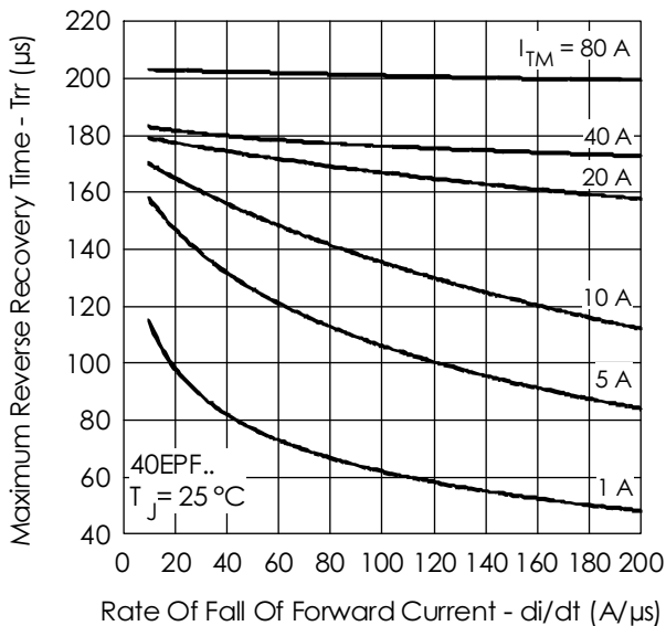
Fig. 8 - Recovery Time Characteristics, T_J = 25^\circ\text{C}
