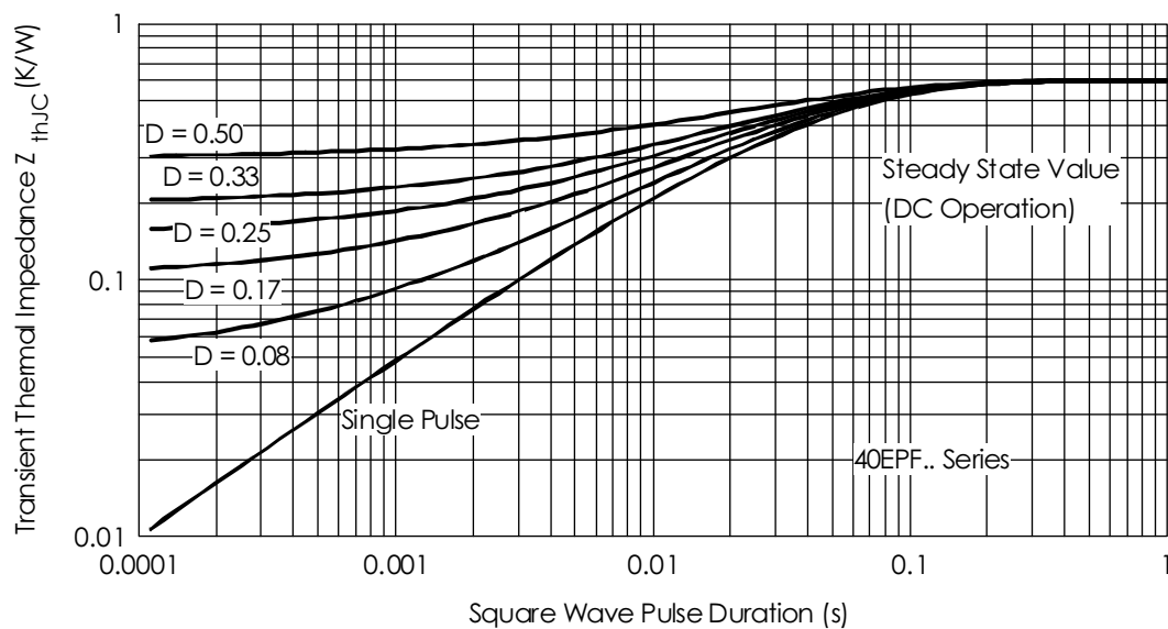
Fig. 14 - Thermal Impedance Z_{thJC} Characteristics
