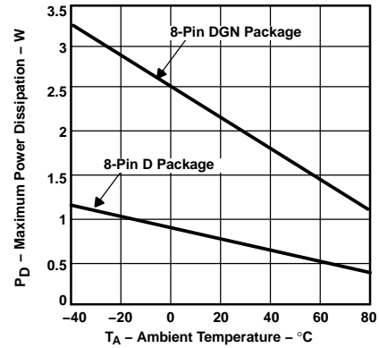
Figure 95. Maximum Power Dissipation vs Ambient Temperature
