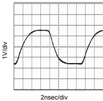
Fig. 19 67.5MHz output waveform (VDD=3.3V, CL=15pF, Ta=25°C)
