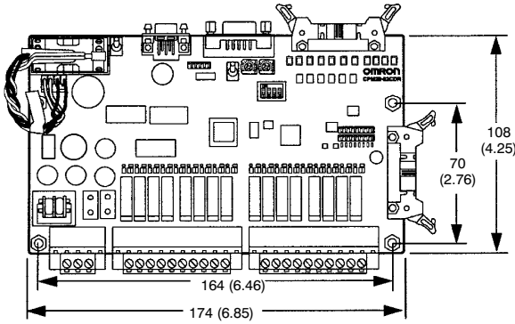
CPM2B-32C□D□-D 32-point Models
