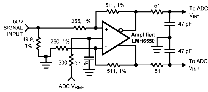
FIGURE 5. Differential Drive Circuit using a fully differential amplifier.
