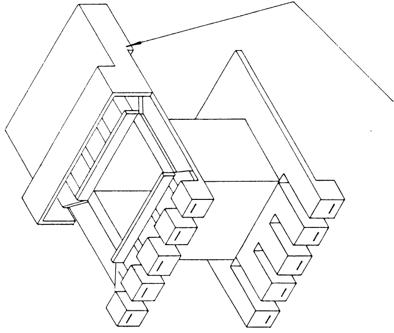
Insulator fitted to one bobbin cheek
