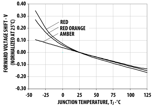
Figure 6. Forward Voltage Shift vs. Junction Temperature
