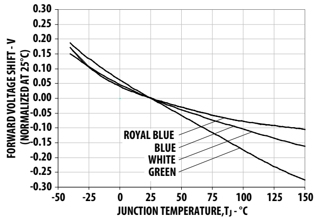
Figure 16. Forward Voltage Shift vs. Junction Temperature
