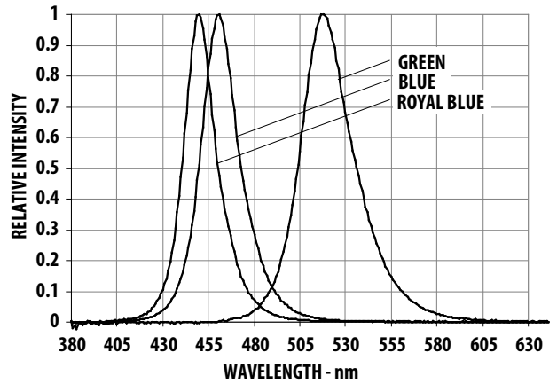
Figure 10. Relative Intensity vs. Wavelength for Blue, Royal Blue and Green
