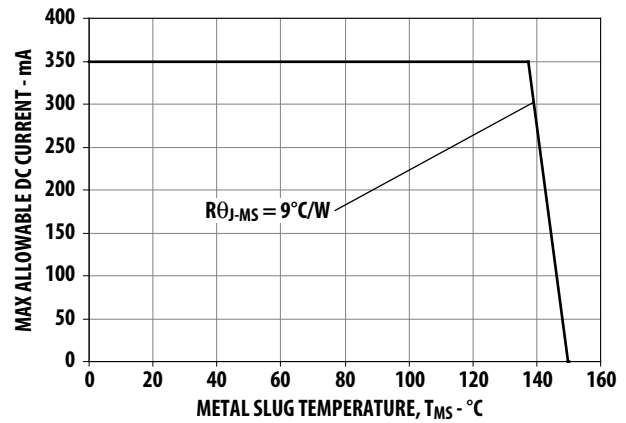
Figure 18. Maximum Forward Current vs. Metal Slug Temperature. Derated based on T JMAX = 150°C, R θJ-MS = 9°C/W.
