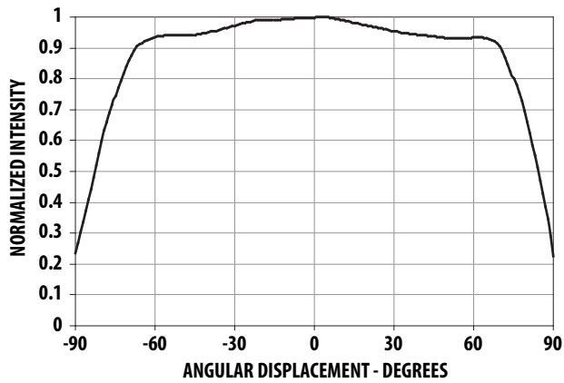
Figure 13. Radiation Pattern for Blue, Royal Blue and Green
