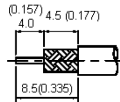
Stripping Dimension
