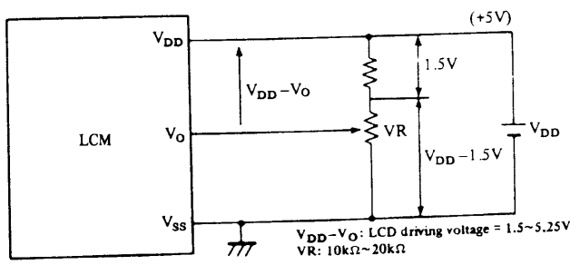
Fig. 4 Power supply
