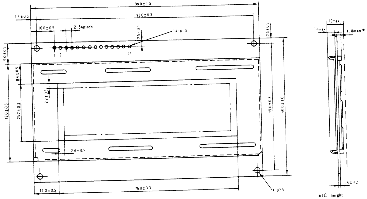
Fig. 2 External dimensions
