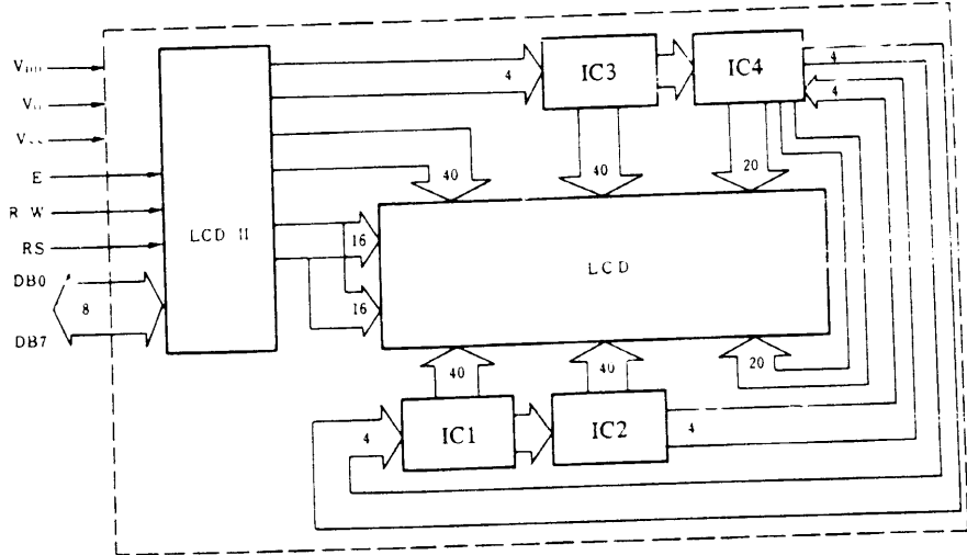
Fig. 3 Block diagram
