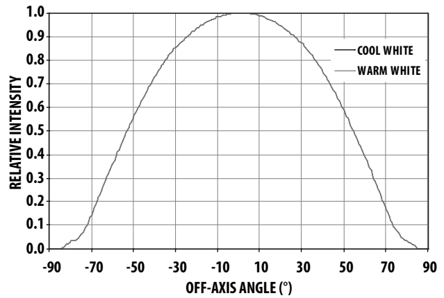
Figure 4. Radiation Pattern
